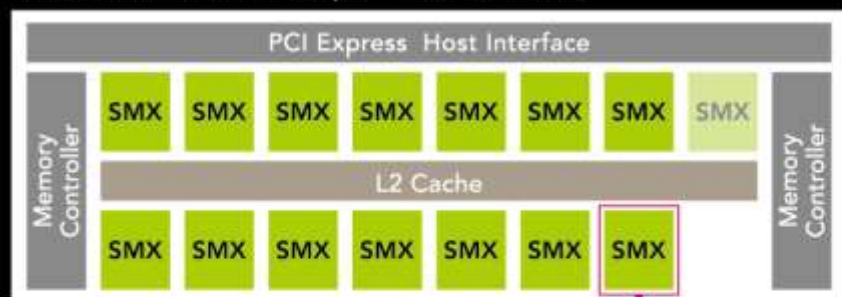
K20X Architecture (Kepler GK110 Core)
