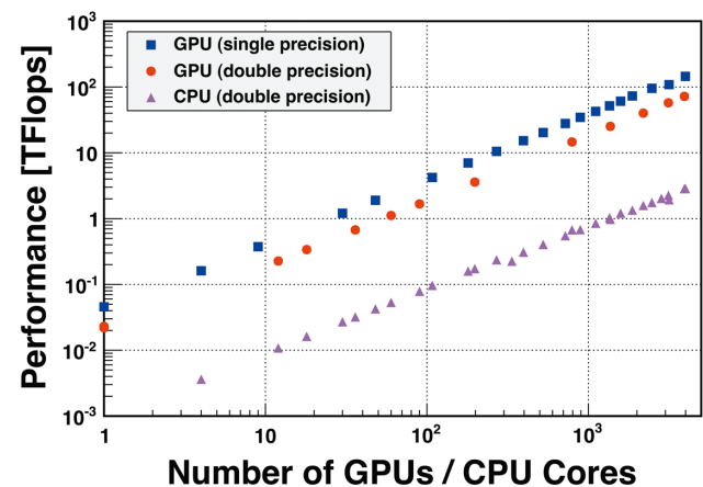
Figure 5 Multi-GPU performance of ASUCA on TSUBAME 2.0 comparing with the CPU.
