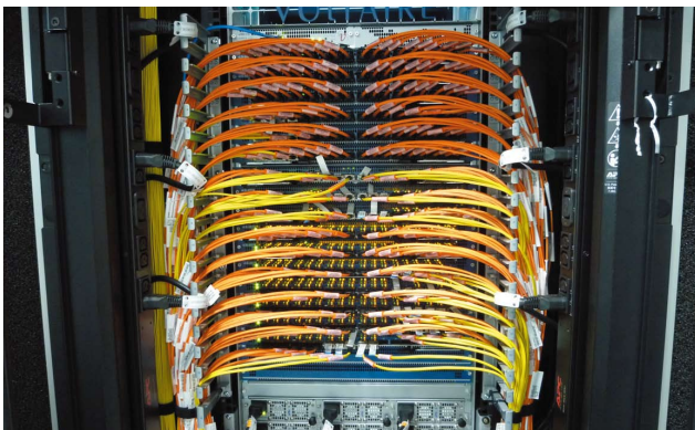
Figure 5 Fiber optic cables are aggregated into the large Infiniband core switch fabric from the the lower-tier edge switches
