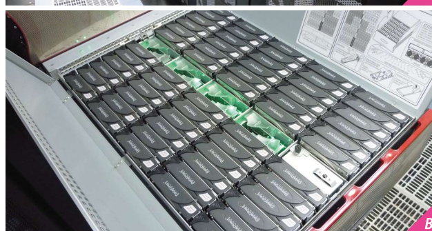
A Figure 7 Various storage servers in TSUBAME 2.0 for Lustre, GPFS, NFS, CIFS, etc.
