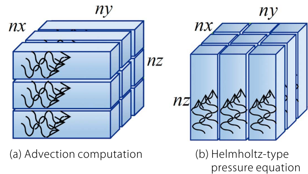
Figure 2 Configuration of the CUDA blocks and marching directions of the threads.
