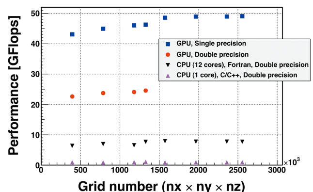
Figure 4 Single GPU performance on a NVIDIA Tesla M2050 of TSUBAME 2.0 and CPU performance of the Intel Xeon X5670.
