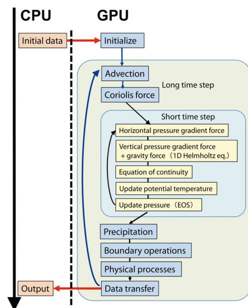
Figure 1 Computational flow diagram of the ASUCA. All the modules inside the short time-step and the long time-step loops are executed on the GPU.
