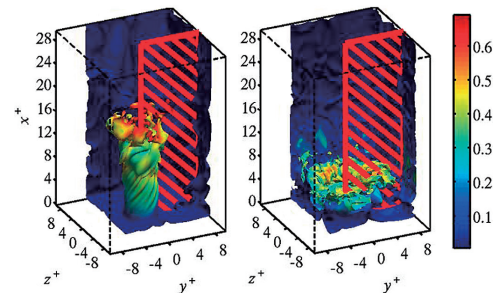
Fig. 8 Typical combustion DNS results of swirl flow stabilised turbulent flames of hydrogen-air combustion. Iso-surfaces: heat release rate. Color: normalised temperature. Left: low swirl number (0.6) case. Right: high swirl number (1.2) case
