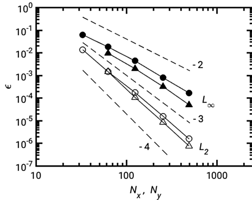
Fig. 5 Error convergence plot of the present IBM obtained from a laminar Taylor-Couette DNS.
